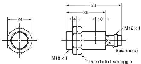
E2A-M18KS08-M1-□□/E2A-S18KS08-M1-□
